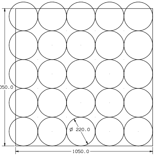
25 BOATS IN A TRADITIONAL MOORING GRID.
