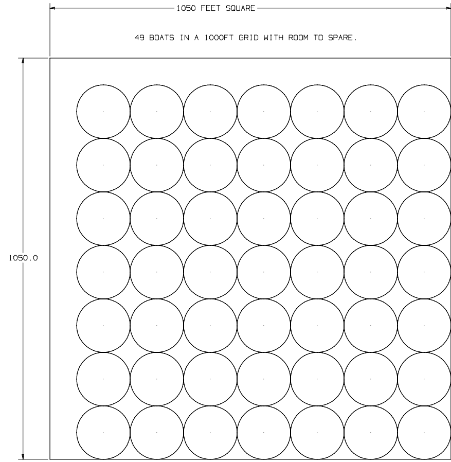
5. SWING CIRCLE FOR HAZELETT ELASTIC MOORING EQUIPMENT AND A 15 FT PENDANT 142 FT.
