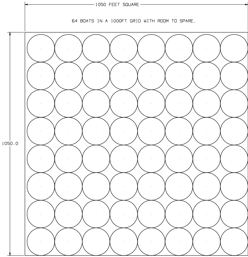
5. SWING CIRCLE FOR HAZELETT ELASTIC MOORING EQUIPMENT AND A 15 FT PENDANT 130 FT.
